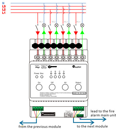
Figure 8. Product Wiring Diagram
