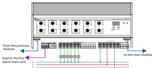
Figure 9. Product Wiring Diagram
