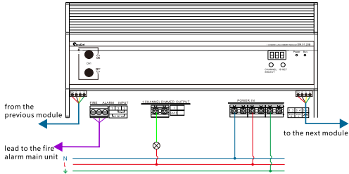
Figure 9. Product Wiring Diagram
