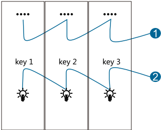
Figuer6.PLC Three Key Smart Panel (With Relay)
