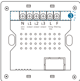
Figuer7.back view
