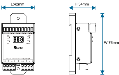
Figure 2. Dimensional Drawing - Front View Figure 3. Dimensional Drawing -Sideview
