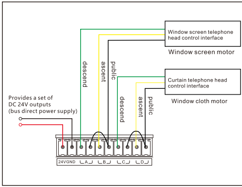
Figure 7. Curtain interface wiring
